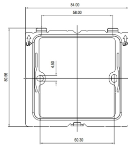
1 FRONT VIEW
