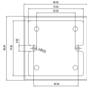
1 FRONT VIEW
