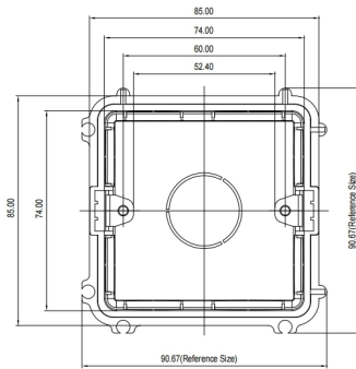
1 FRONT VIEW
