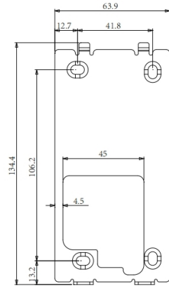
5 TOP VIEW
