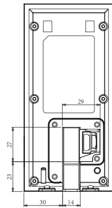
4 BACK VIEW
