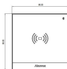
1 FRONT VIEW
