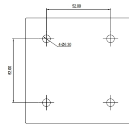
4 BACK VIEW
