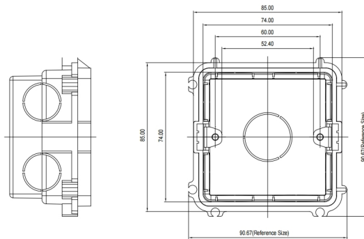
1 FRONT VIEW
