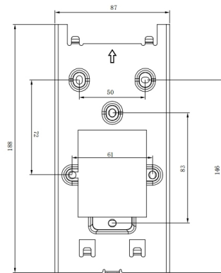
① FRONT VIEW
