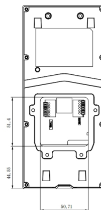
④ BACK VIEW
