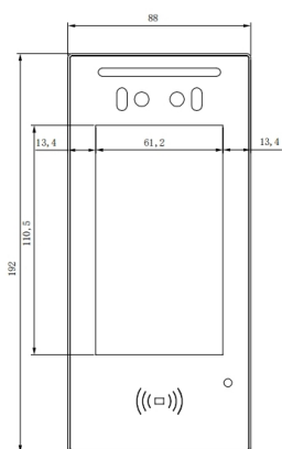
① FRONT VIEW
