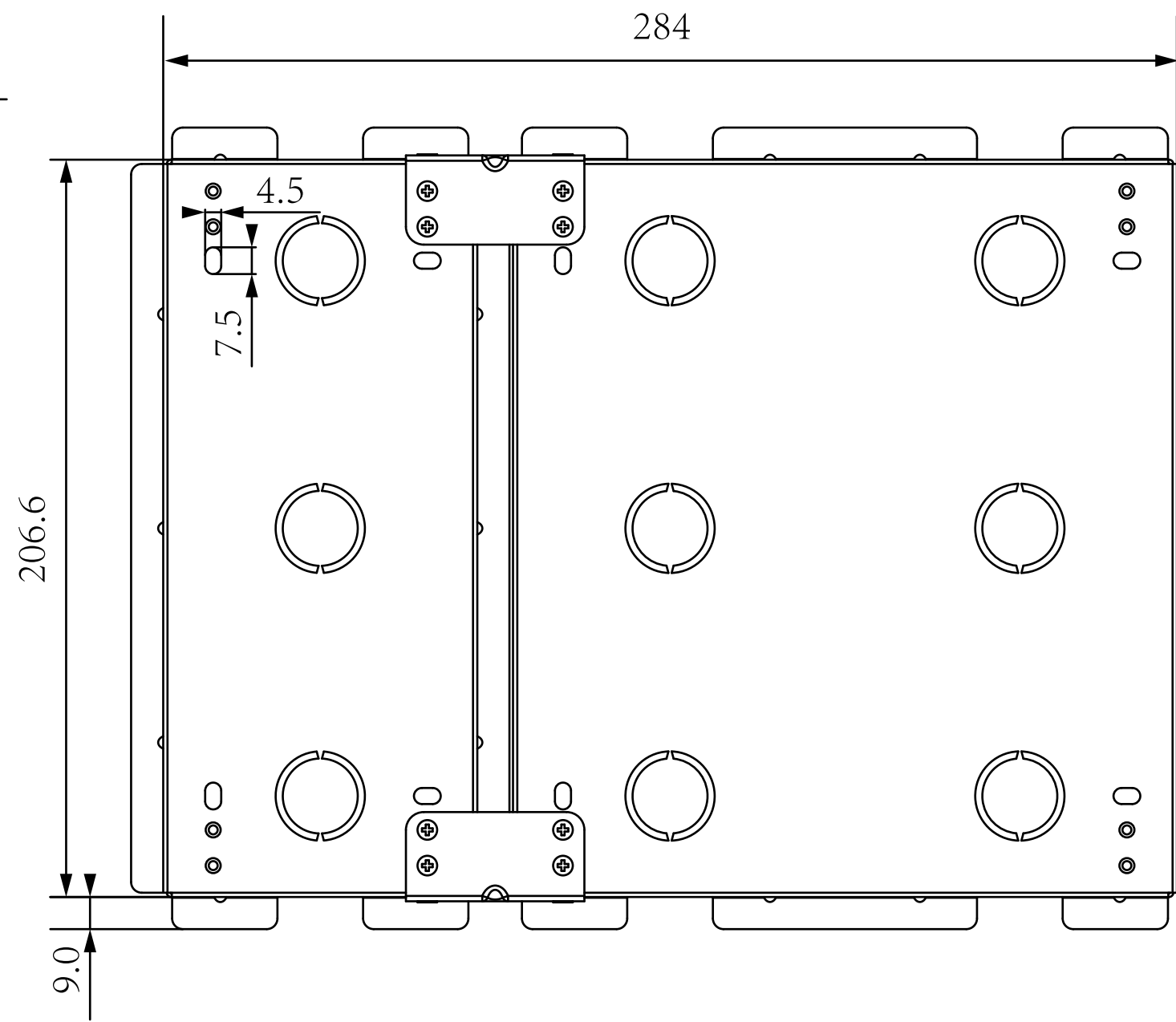
④ BACK VIEW
