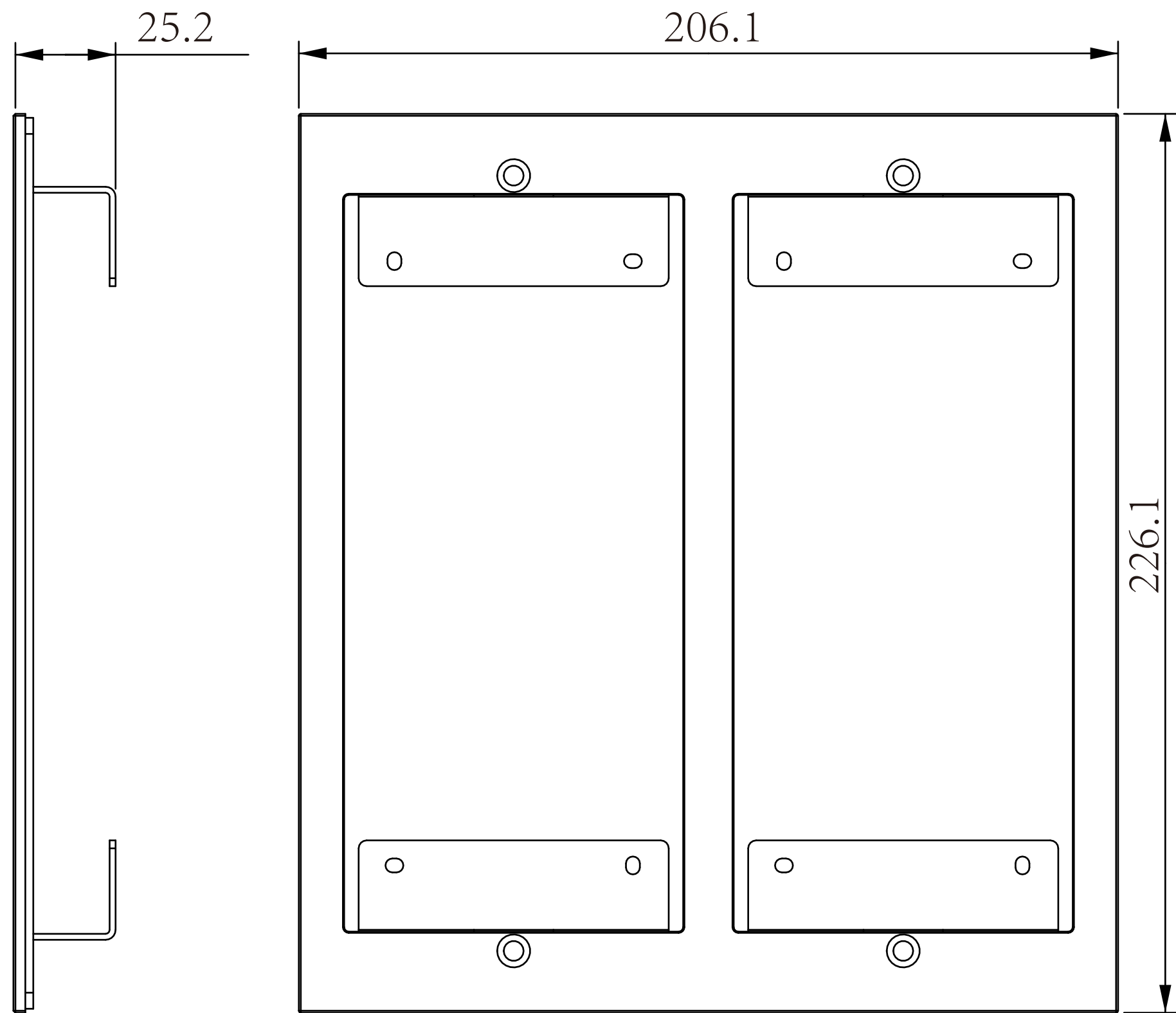
① FRONT VIEW
