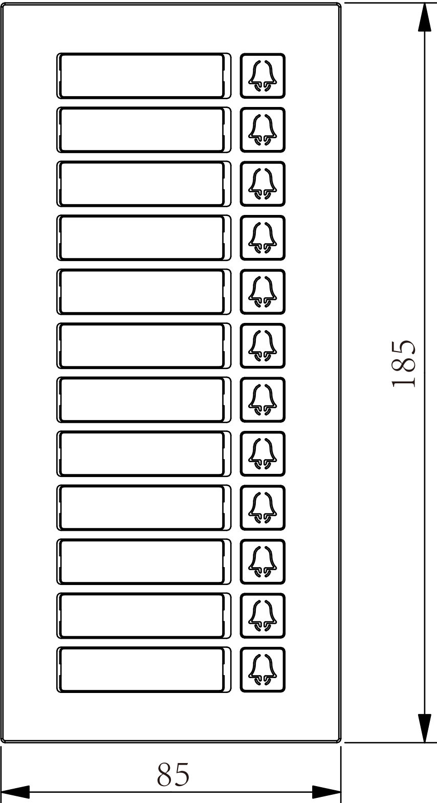
① FRONT VIEW
