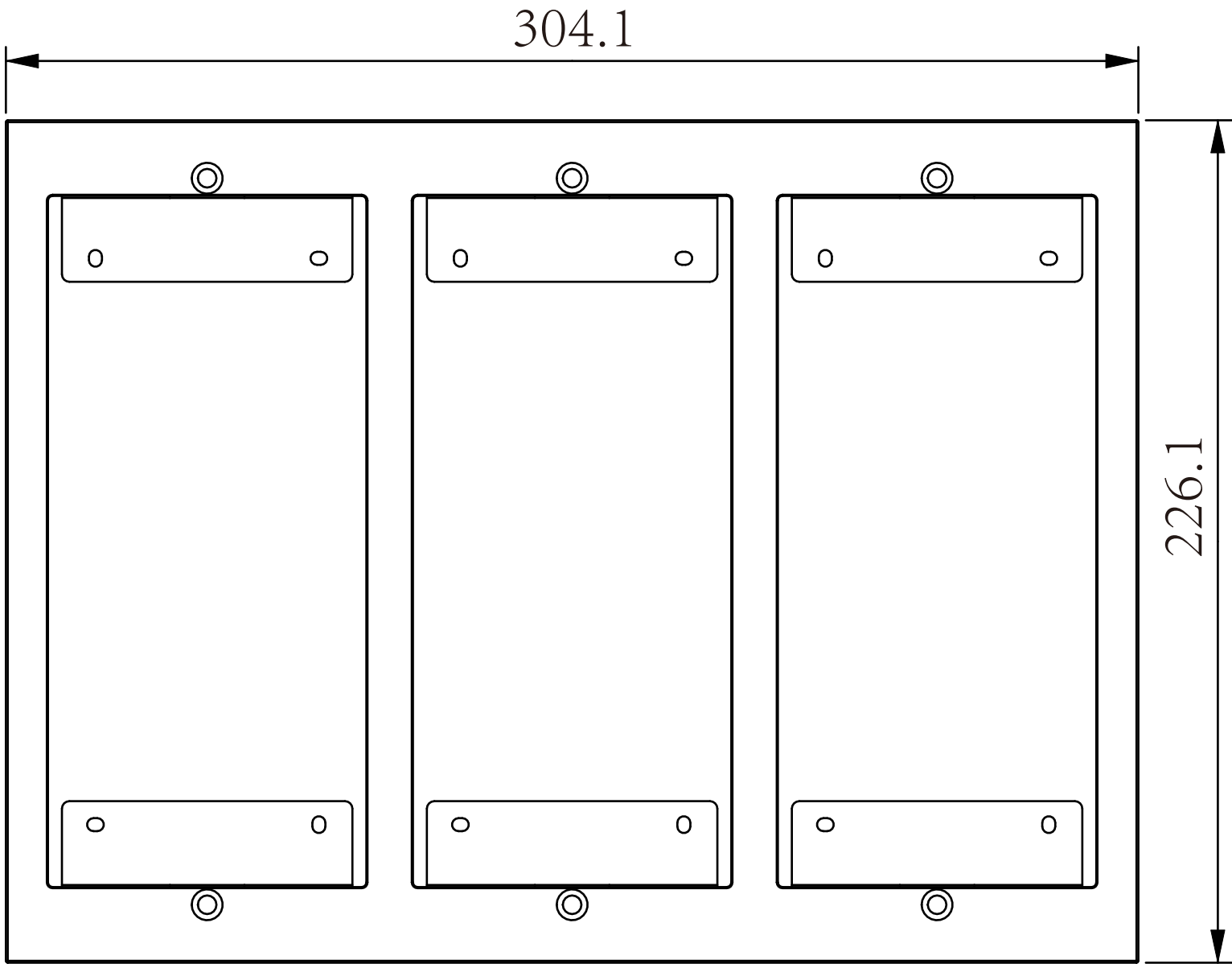
① FRONT VIEW
